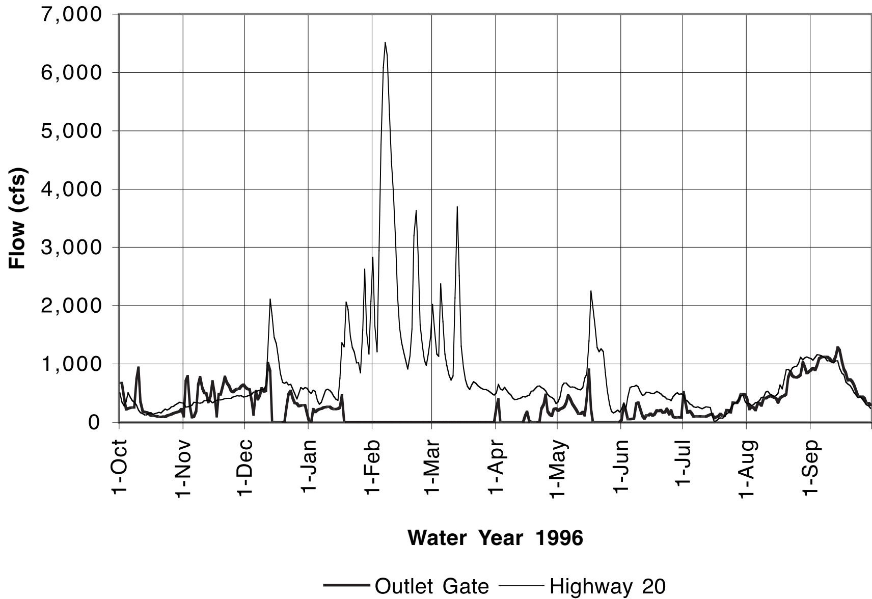
Figure 2-20 Daily Flows in Colusa Basin Drain at Highway 20 and the Outlet Gate to the Sacramento River during Water Year 1996
