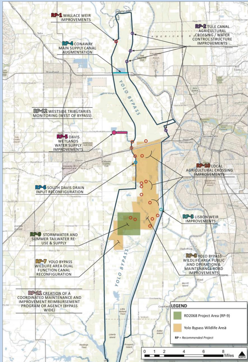
Notes: cbec Yolo Bypass Drainage and Water Infrastructure Projects Project No. 12-1039 CREATED BY: SPW Yolo Bypass Drainage Study Figure 1
