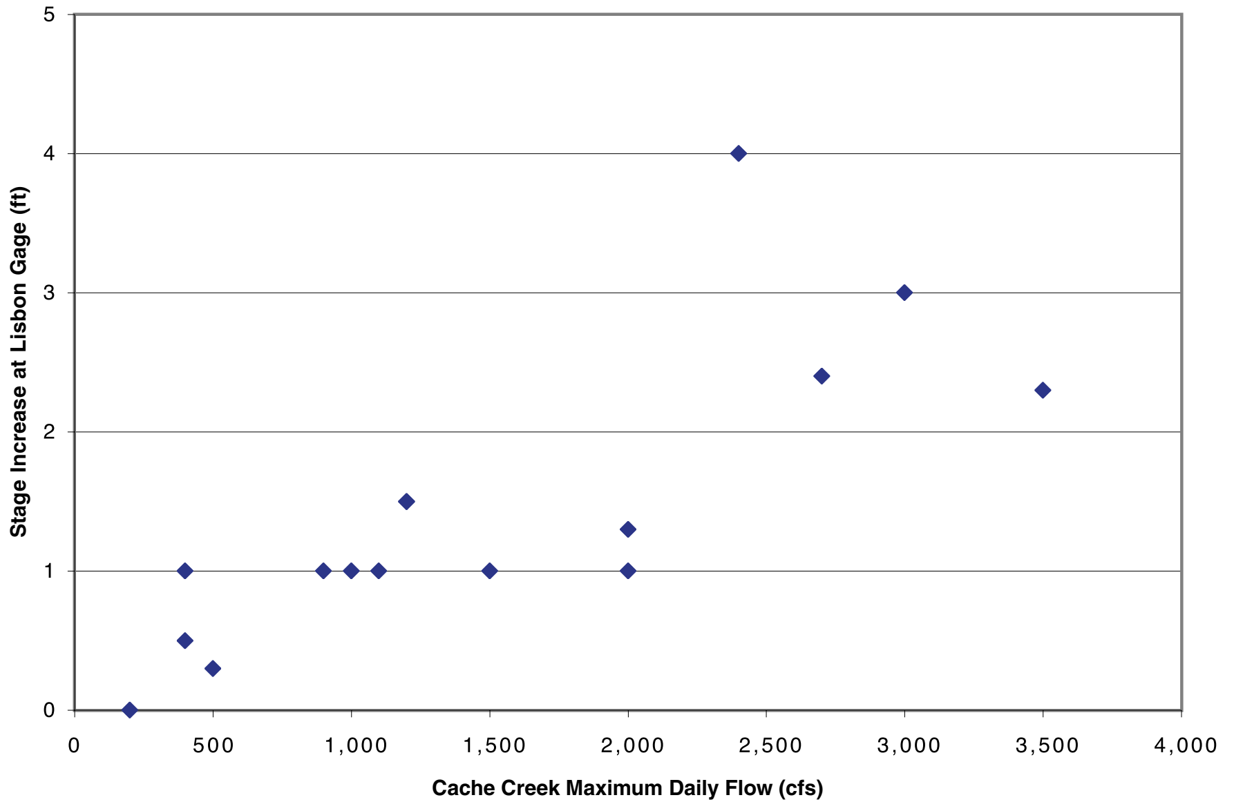
Figure 2-18 Effect of Cache Creek Runoff Events on Stage at Lisbon Gage in Years Without Fremont Weir Spills
